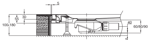
with BETTE INSTALLATION SYSTEM FLUSH-TO-FLOOR
