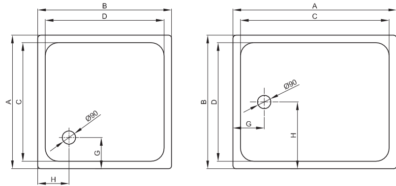
shower tray with shank length \geq 100 cm
