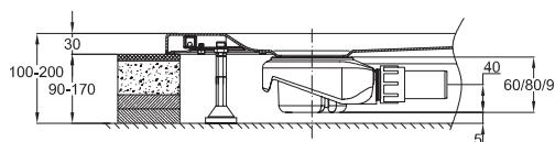
with BETTE FOOT-SYSTEM
