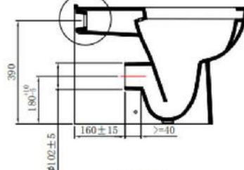
SIDE VIES
