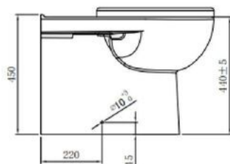
SIDE VIES
